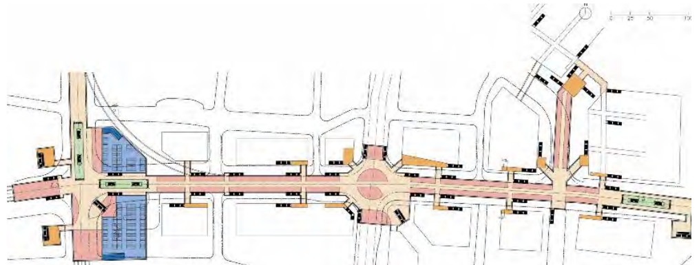
Plan view of the underground space in the key area
